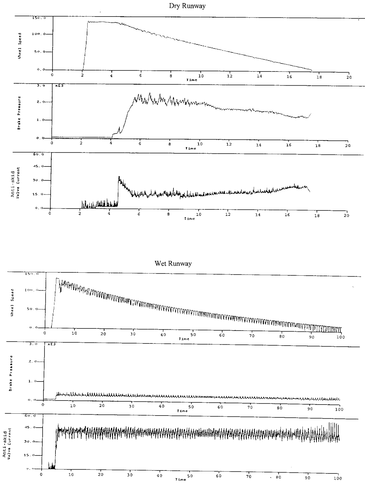
Figure 4-7. Anti-Skid System Response Characteristics: Fully Modulating System
