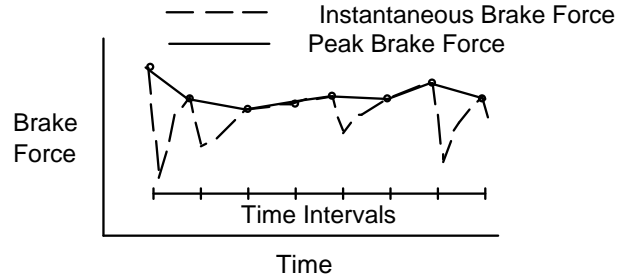
Figure 4-8. Instantaneous Brake Force and Peak Brake Force
