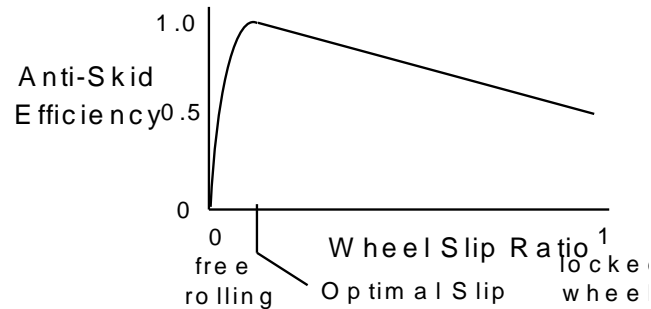
Figure 4-9. Anti-Skid Efficiency–Wheel Slip Relationship
